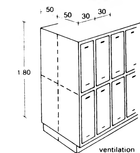
⑫ Two-level row of lockers
